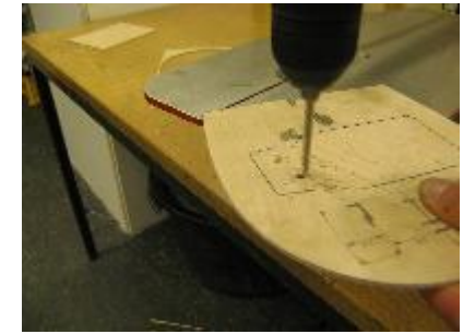
Bag 7-18: Cockpit
