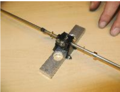
Bag 8-03: Rotor
