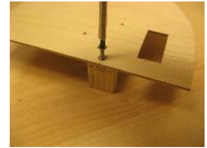
Bag 7-34: Cockpit
