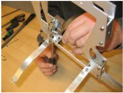
Bag 2-7: Skids
