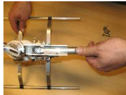
Bag 5-4: Tailboom
